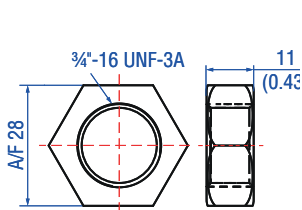
Hex jam nut 3/4\"-16 UNF-3A Part no. 500 015
