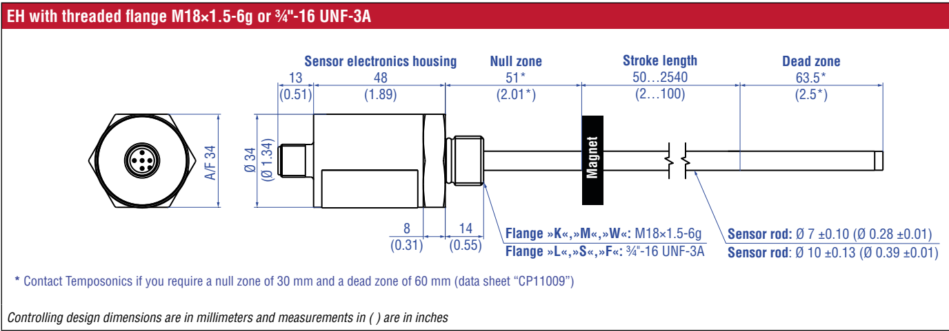
Fig. 3: Temposonics® EH with ring magnet
